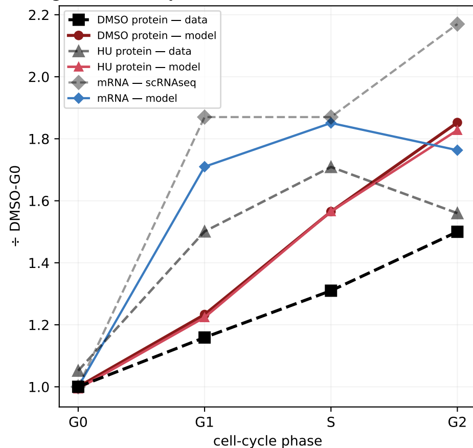
(B) Best fit vs data — DMSO & HU protein + mRNA (HU longer-S boost captured; Pal/RO excluded — model 2N-collaps@around kEZbas 0.004 / kDeEZ 0.0005; blue→red = low→high value)
