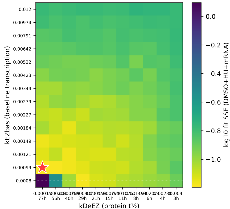
(A) Fine fit landscape — ★ best kEZbas=0.00099, kDeEZ=0.00015 ( t_{1/2} 77h)
