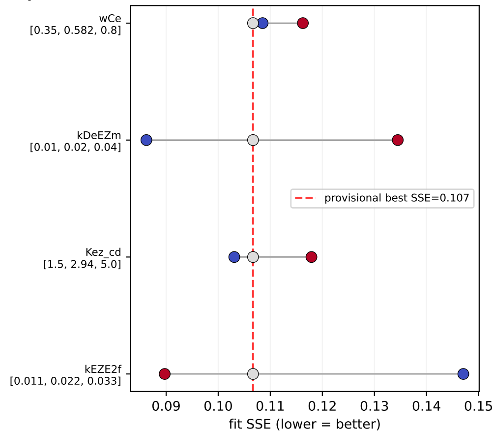
(C) Secondary rate-var sensitivity (around kEZbas 0.004 / kDeEZ 0.0005; blue→red = low→high value)
