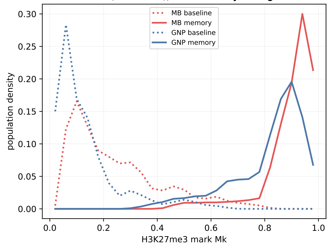
(C) Mark distribution: memory mark piles up at M_k \sim 1 (saturated), baseline stays low/graded
