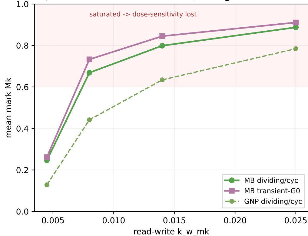
(B) The mark SATURATES the dividing population too (rebuild beats division-dilution) -- no graded window
