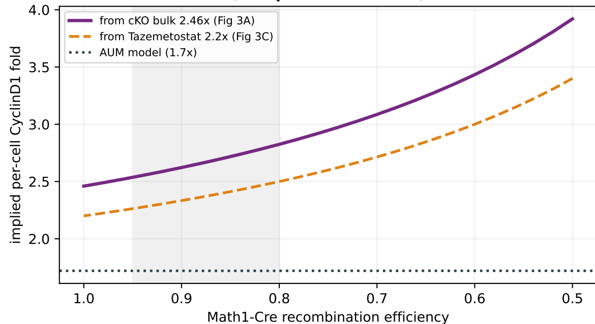
(a) The bulk cKO fold UNDER-estimates per-cell de-repression (escaper cells dilute it)
