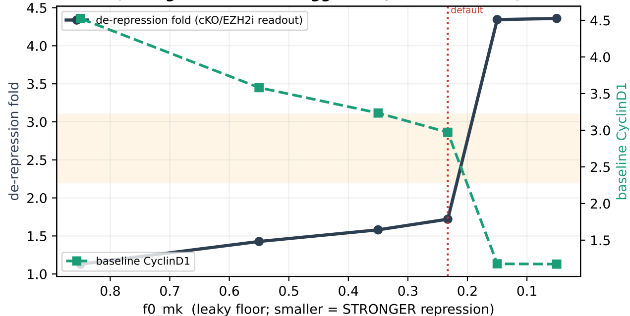
(b) Model feedback strength sets the measurable fold (stronger feedback = bigger fold, lower baseline)
