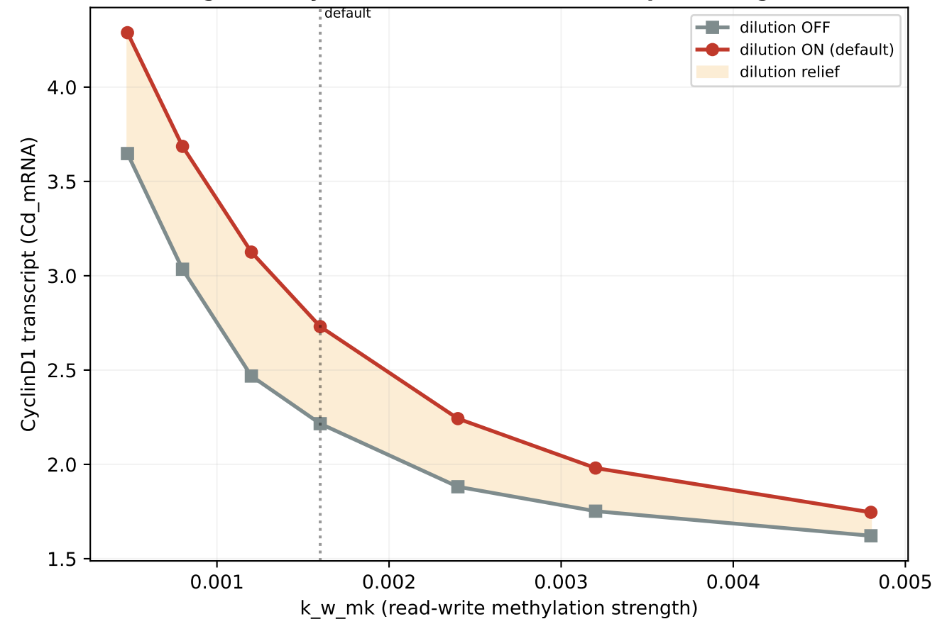
(D) Deposition vs dilution stronger methylation ↓ Cd, but dilution keeps clawing it back
