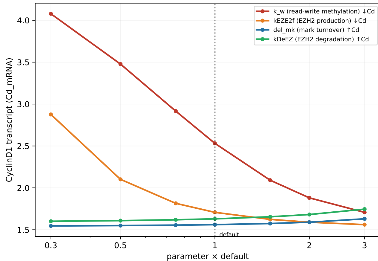
(C) Control parameters of the tension deposition knobs ↓ CyclinD1; removal knobs ↑ CyclinD1
