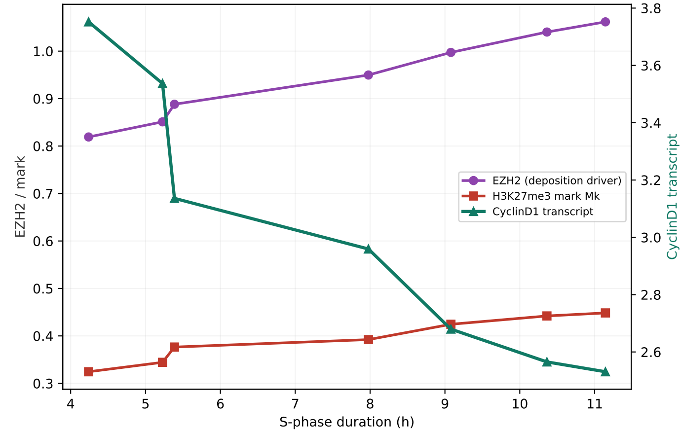
(D) Deposition vs dilution stronger methylation ↓ Cd, but dilution keeps clawing it back
