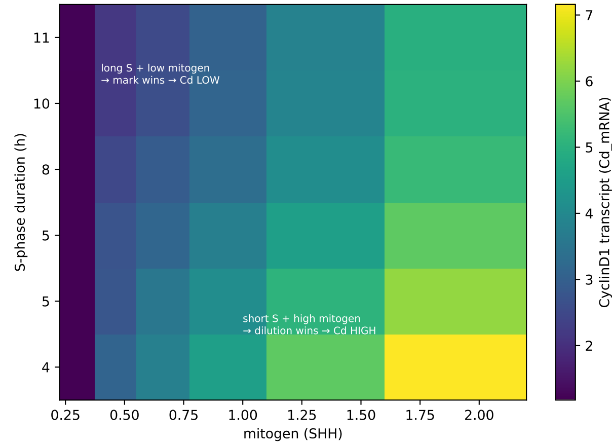
(C) Control parameters of the tension deposition knobs ↓ CyclinD1; removal knobs ↑ CyclinD1
