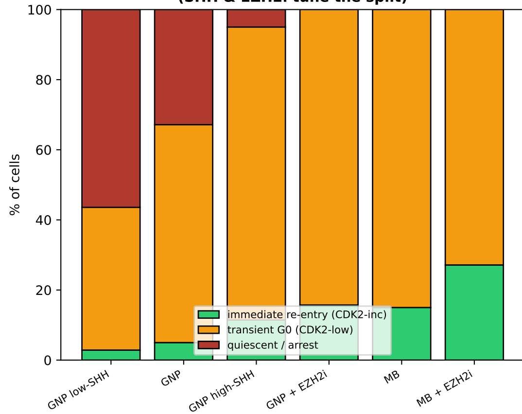
(a) Proliferation-quiescence bifurcation (SHH & EZH2i tune the split)
