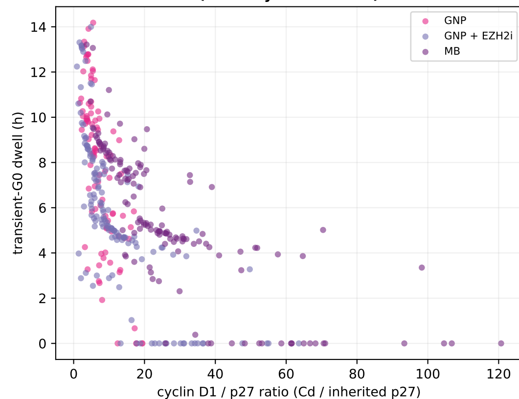
(c) G0 dwell set by the cyclin D1/p27 ratio (Fan-Meyer threshold)
