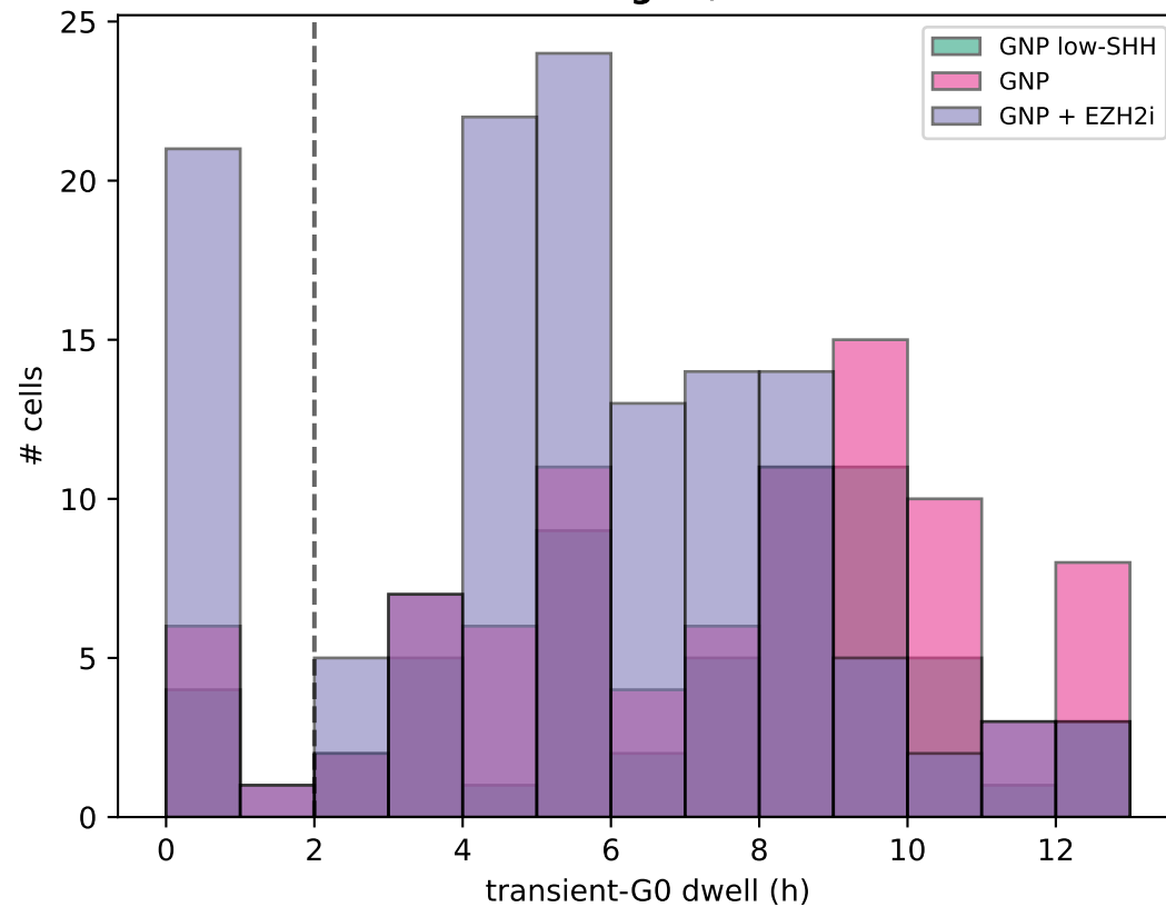
(b) G0 dwell-time distribution shifts with mitogen / EZH2i
