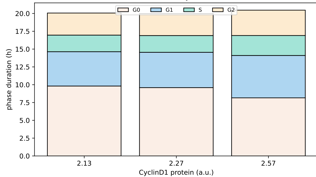
(b) Phase partition vs CyclinD1 (G0 shrinks into G1/S; period ~constant)
