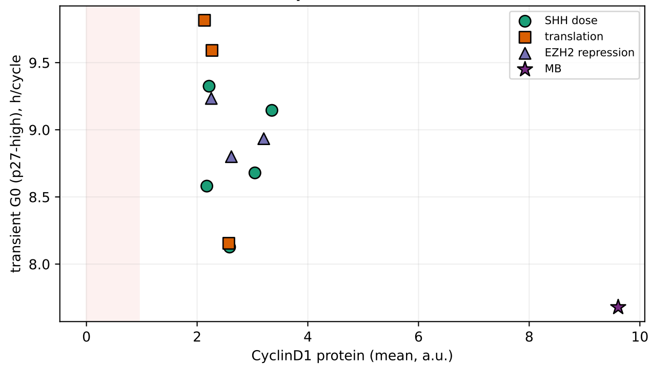
(a) CyclinD1 sets transient-G0 duration (all knobs collapse; arrest below threshold)
