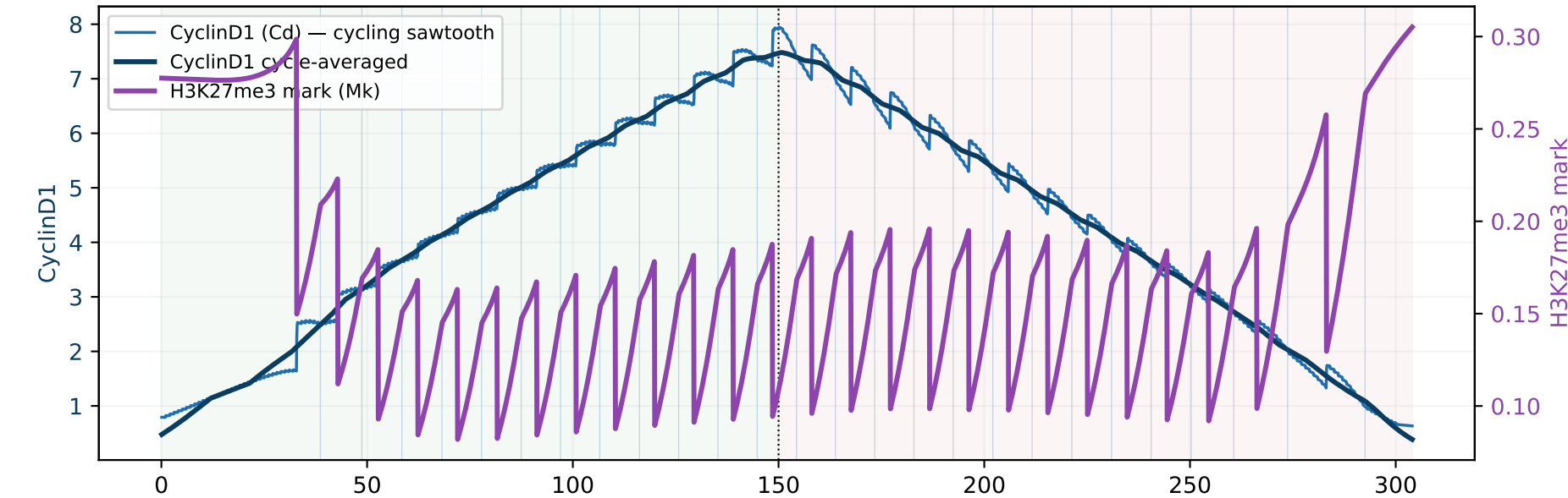
(C) EZH2 writer + divisions — 12 divisions on UP-leg, 14 on DOWN-leg
