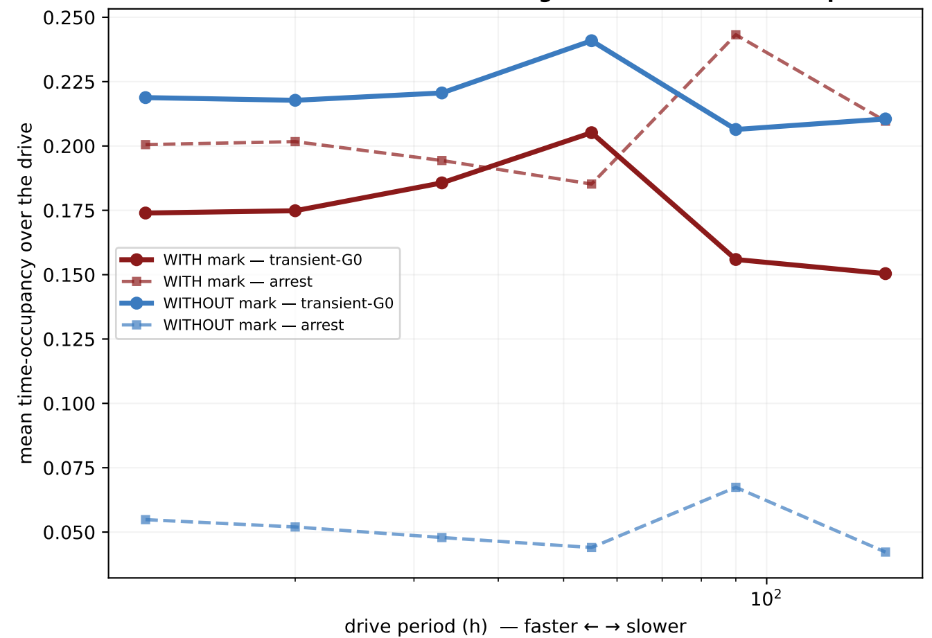
(D) MEAN transient-G0 (solid) & arrest (dashed) under fluctuations WITH vs WITHOUT — does the mark change how much time cells spend in G0?
