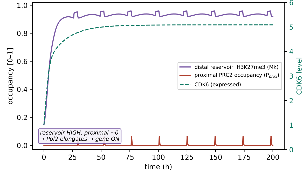
(A) Marked but expressed — cycling cell
