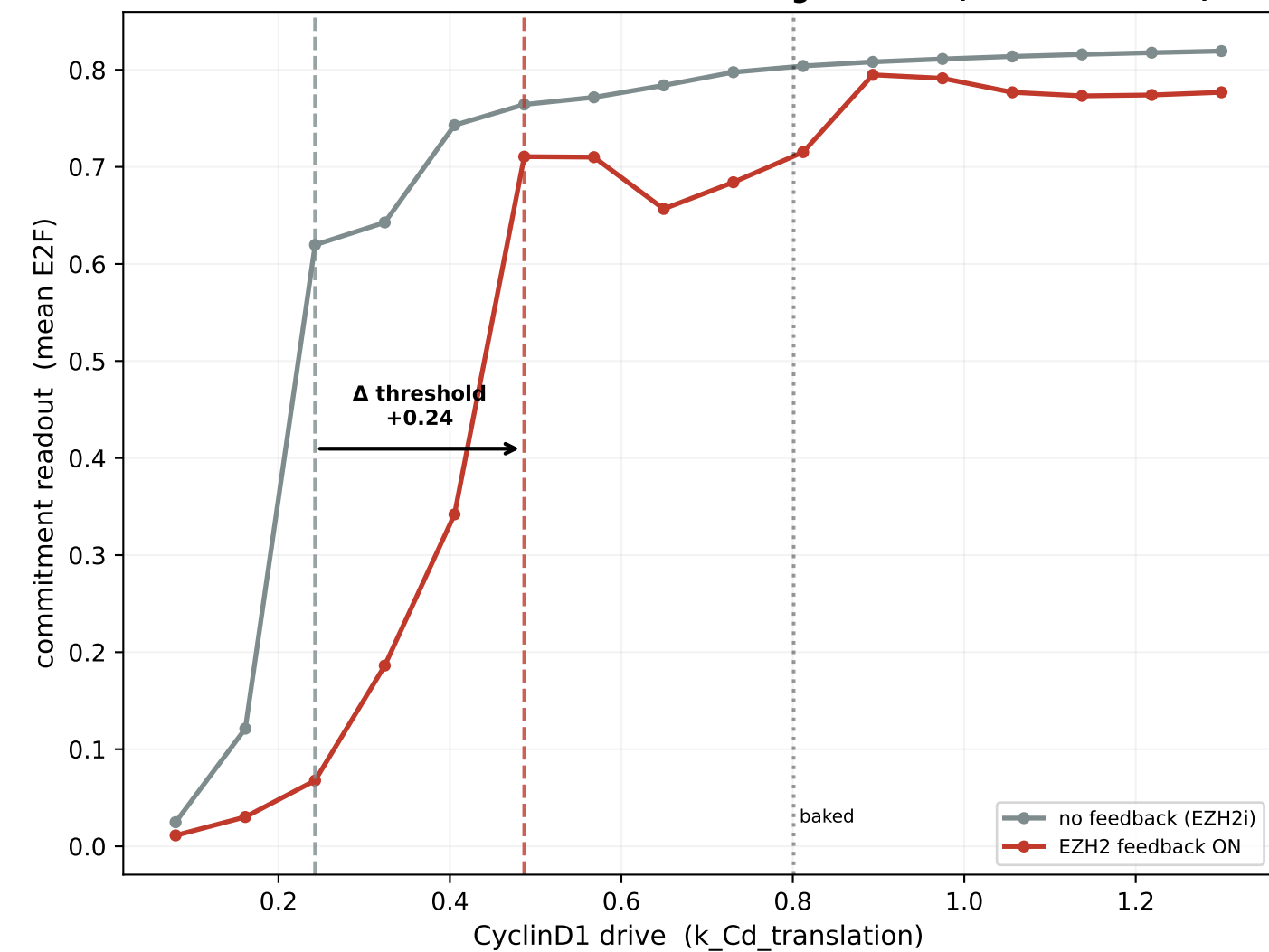
(C) Proliferation-quiescence bifurcation vs CyclinD1 drive EZH2 feedback shifts the threshold to higher drive (dashed = onset)
