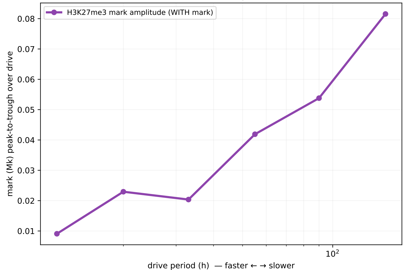
(D) The mark is the slow filter: its own oscillation is small for FAST drives (can't follow) and grows for SLOW drives
