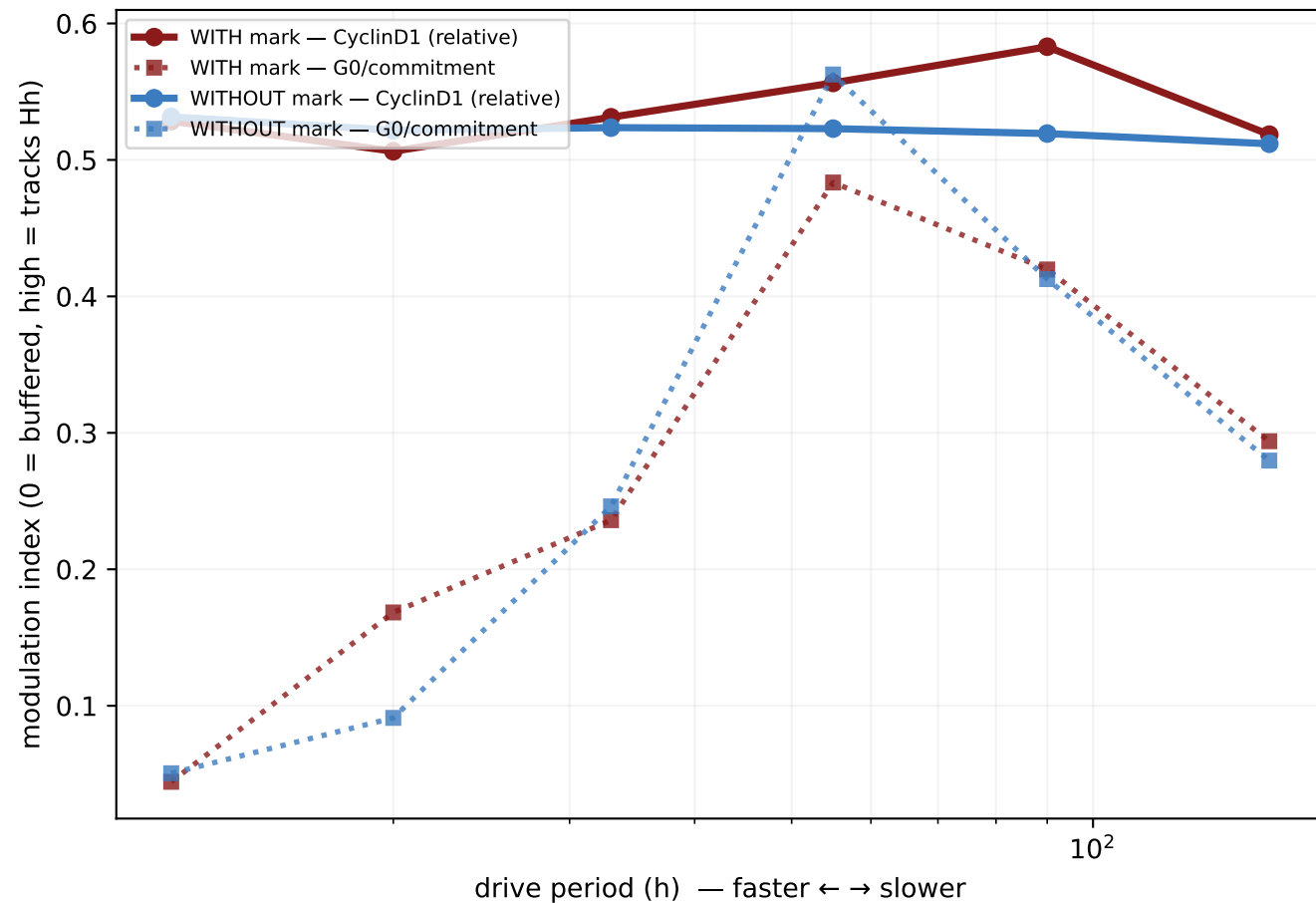
(C) CyclinD1 relative swing ≈ equal & flat (mark SCALES, no low-pass); G0/commitment (dotted) IS low-pass filtered (buffered vs fast) but ~EQUAL WITH/WITHOUT → the buffering is the cell cycle + commitment switch, NOT the mark
