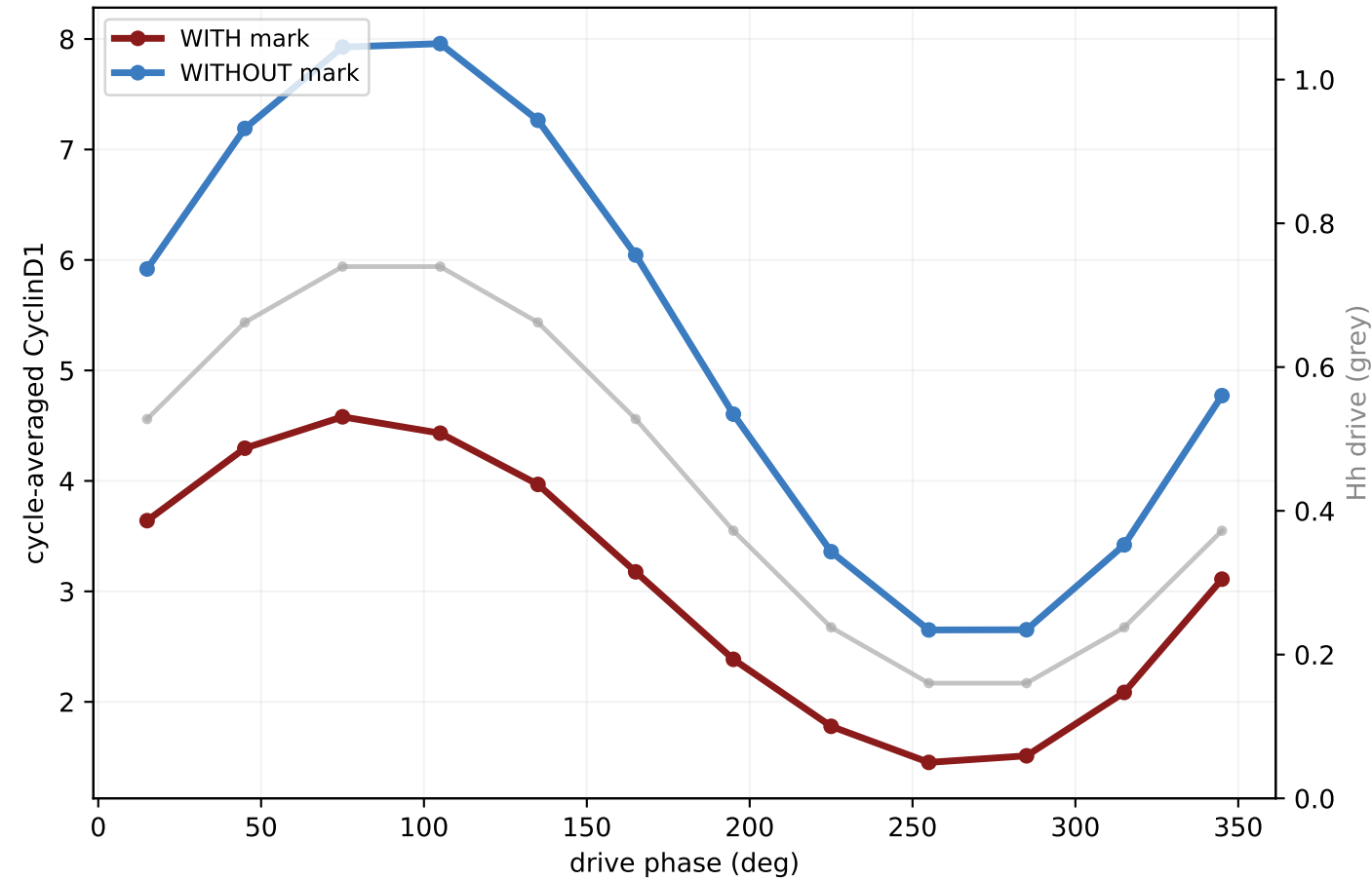
(B) SLOW fluctuation (T=150 h): CyclinD1 tracks the drive (both)
