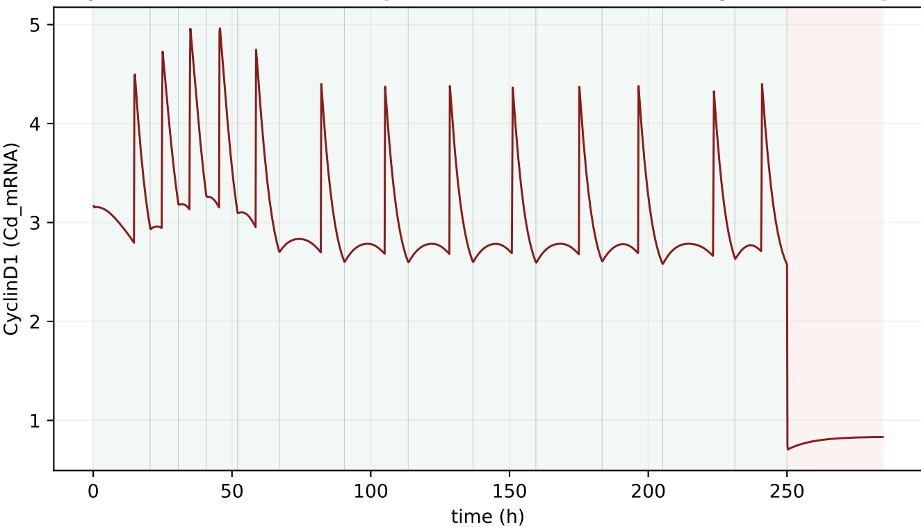
(B) CyclinD1 sawtooth — envelope DECLINES as the mark charges (harder to push)
