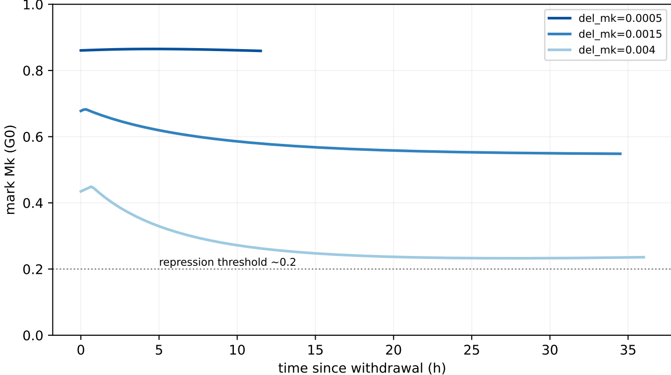
(D) BATTERY DISCHARGE in G0 — durability ( \text{del\_mk} ) sets the memory duration
