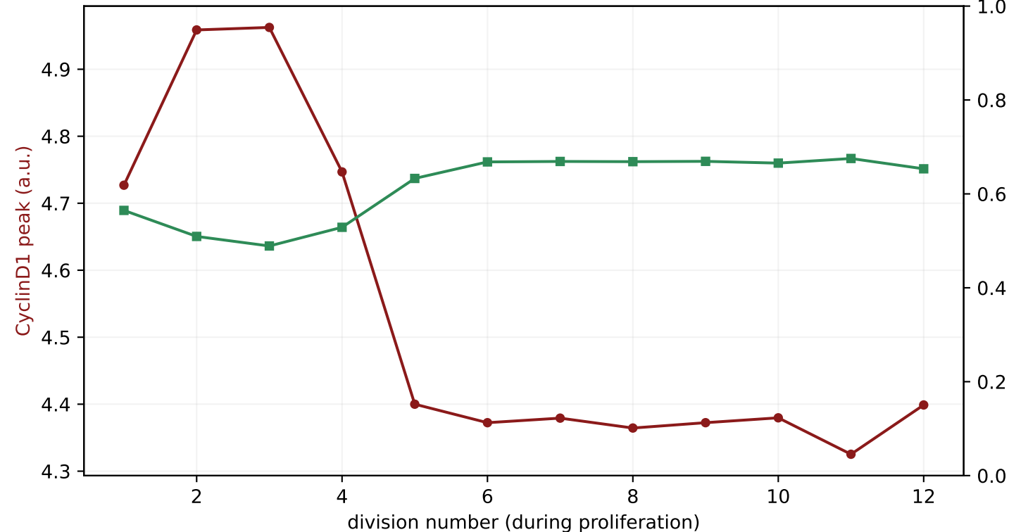
(C) "Harder to push": CyclinD1 peak falls as H3K27me3 charges over divisions
