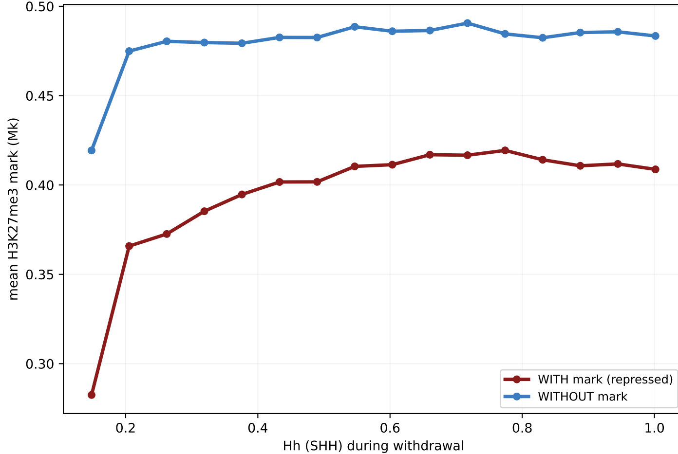
(C) Mean mark FALLS as Hh withdraws — restoration is CYCLE-GATED
