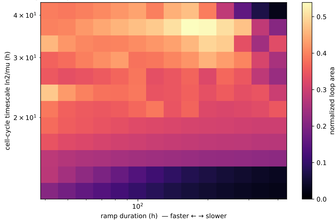
(C) mu (dilution frequency / cycle period)
