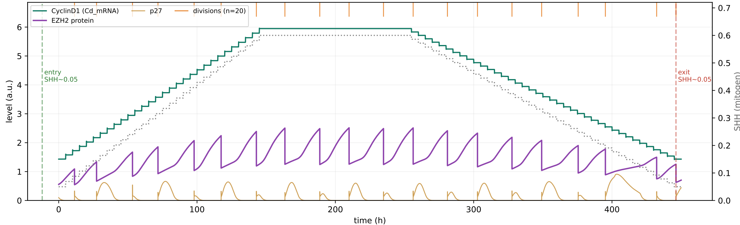
WITHOUT H3K27me3 repression (f0_mk=1.0) — no mark: CyclinD1 tracks mitogen directly
