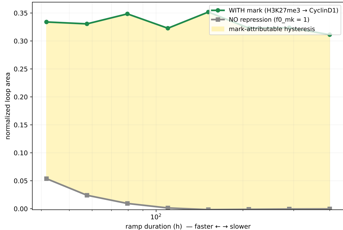
(B) Loop area vs ramp speed: with vs without the mark the gold gap is the hysteresis the H3K27me3 mark contributes
