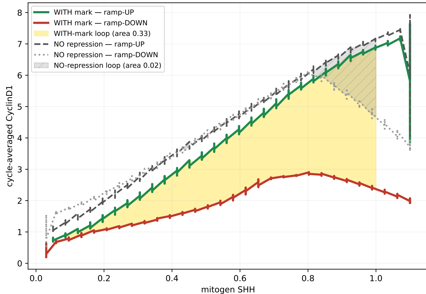
(A) CyclinD1-SHH loop at a fast ramp (58 h) the mark OPENS the loop; without it up & down nearly coincide
