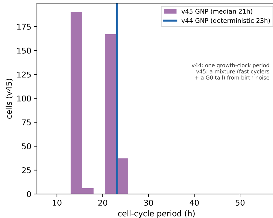
B Period: deterministic vs distribution
