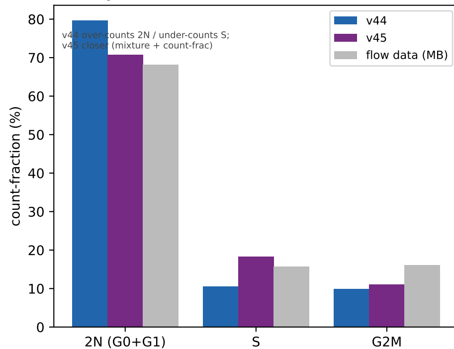
A MB phase fractions (vs data)
