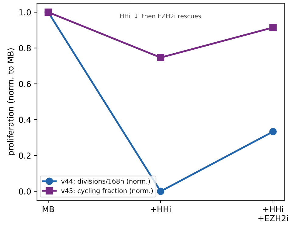
C Rescue: both reproduce it
