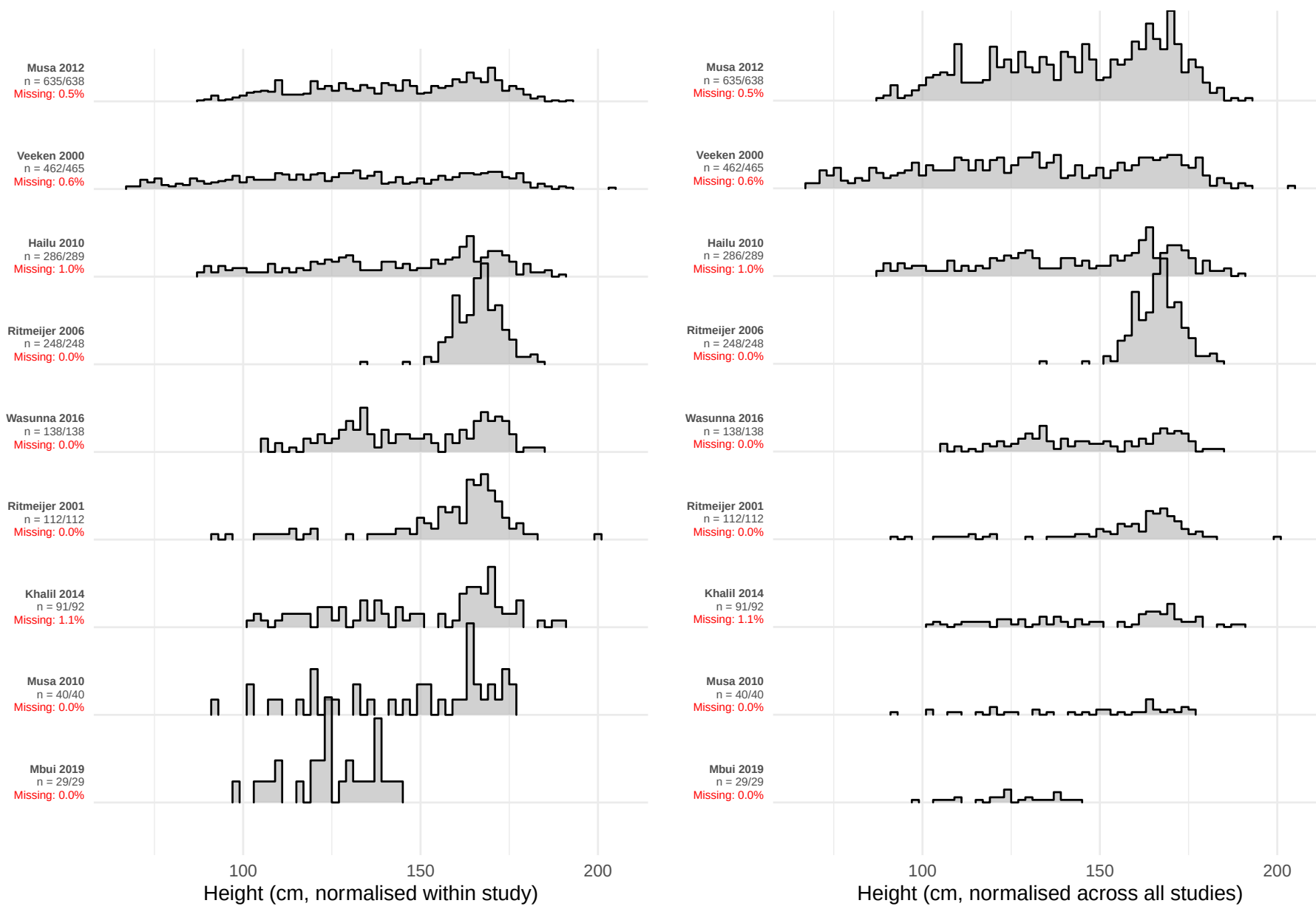
Figure D.3: Distribution of height across studies from East Africa. Missing data described by study.
