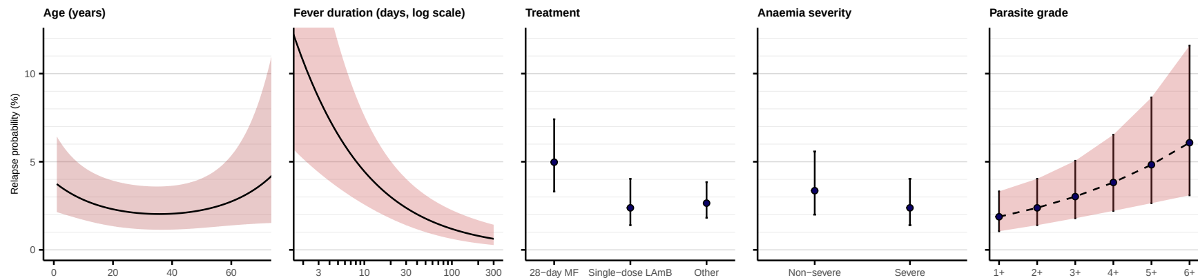
Figure 4.9: Adjusted associations between final predictors and predicted relapse probability, as estimated from the final ISC prognostic models. Probabilities were calculated from optimism-adjusted models and following logistic recalibration (intercept-term only) to data contributed from Sundar 2019[96]. Where not varying in the plot, predictions are standardised to a representative reference participant: median age (18 years), median fever duration (30 days), treated with 10 mg/kg single-dose liposomal amphotericin B, with severe anaemia, and — for the model including parasite grade — a median parasite count of 2+.
