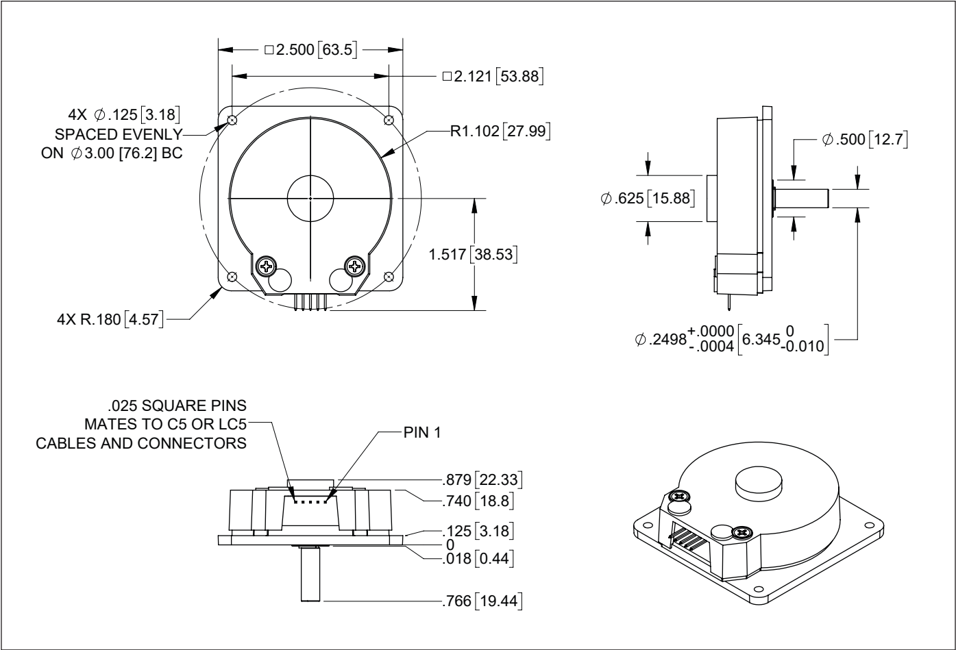
H3 Ball Bearing Rotary Shaft Encoder
