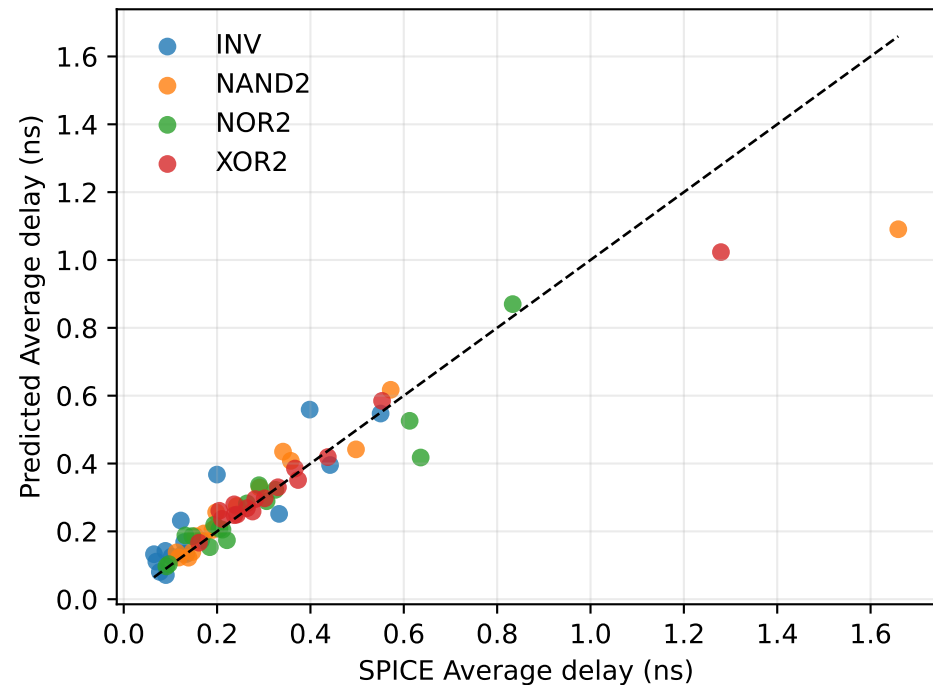
Predicted vs SPICE on held-out primary SPICE dataset rows
