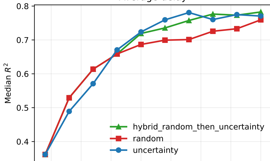
Average delay
