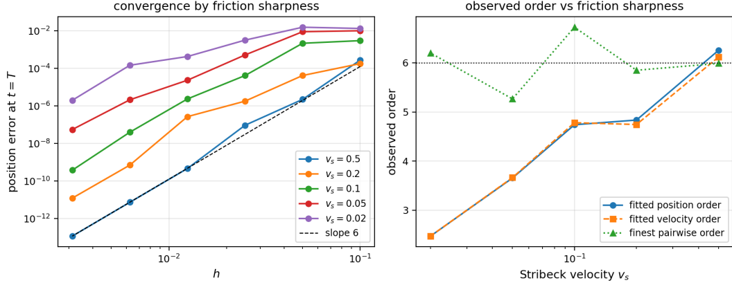
Figure 5: Friction sweep on the chain: position error against step size for five Stribeck velocities (left) and fitted orders against v_s (right).
