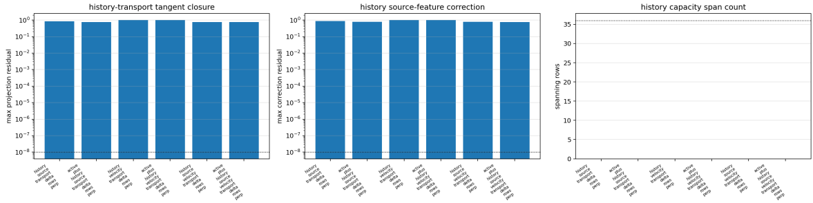
Figure 18: Higher-order/nonlocal capacity audit. Third finite-difference source features and same-case cross-step source deltas still do not span the local lower-pair correction.
