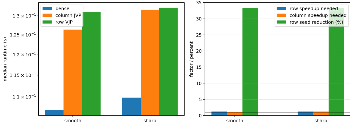
Figure 25: Sparse speed gap audit. Row-VJP reduces the seed count but is not yet a stable wall-clock improvement over dense jacfwd .
