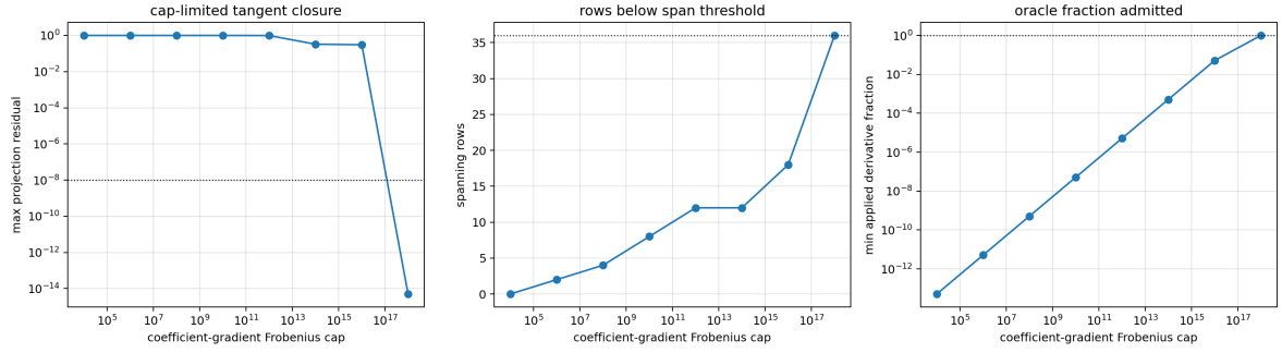
Figure 13: Bounded-gradient cap sweep. The local derivative-aware oracle is capped by a global Frobenius gradient budget. Practical caps recover only part of the local tangent span, while all local spans require cap 10^{18} .
