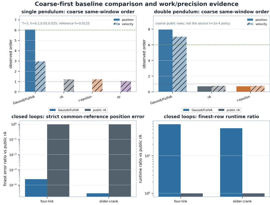
Figure 10: Coarse-first baseline and work/precision diagnostics. The top panels compare observed order on the same coarse window for the single and double pendula. The lower panels use the strict common-reference closed-loop summaries for four-link and slider-crank, with all plotted rows evaluated against the same finite accepted-method endpoint reference at h_{\text{ref}} = 0.0125 . These panels document coarse-first diagnostics and work/precision availability, but they are not an external-superiority claim and do not replace the unresolved original source-policy campaigns.
