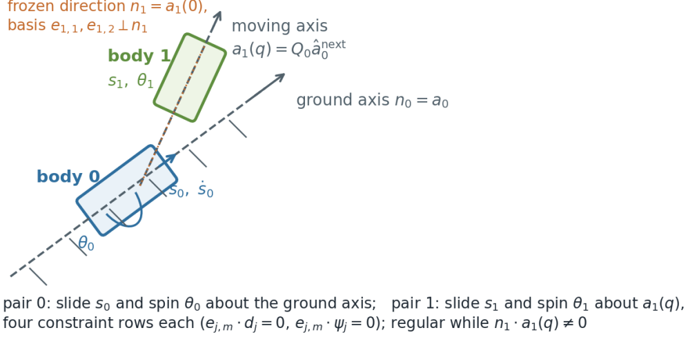
Figure 1: The two-body chain: body 0 slides and spins along the fixed ground axis, body 1 slides and spins along the axis a_1(q) carried by body 0; the second pair keeps its sliding direction n_1 and its basis e_{1,m} frozen at their t = 0 values.
