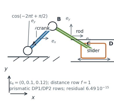
Figure 3: Coordinate-oriented mechanism schematics and lower-pair constraint inventory for the four ASME-style examples. Each panel shows the global coordinate frame, named joints, the principal moving bodies, the driver where applicable, and the CD/DP1/DP2/D constraint vocabulary used by the FullVA rows. Exact body-fixed point and direction vectors are listed in the text immediately preceding the figure.
