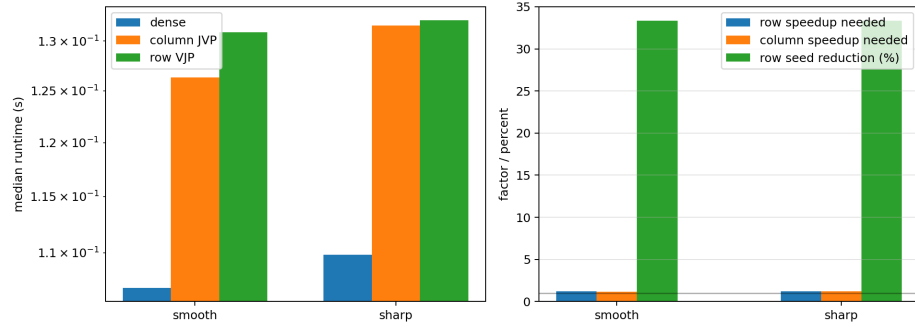
Figure 7: Sparse backend speed-gap diagnostic. The sparse structure is correct and quantified, but dense jacfd remains faster in the recorded wall-clock evidence.
