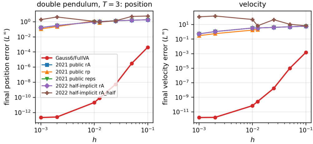
Figure 8: Double pendulum over the public horizon T = 3 : final position (left) and velocity (right) errors of Gauss6/FullVA and of the public absolute-coordinate codes against the common h = 10^{-4} reference.
