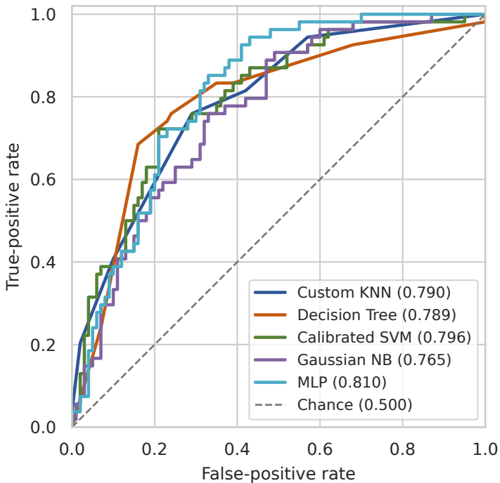
ROC curves on the held-out test set
