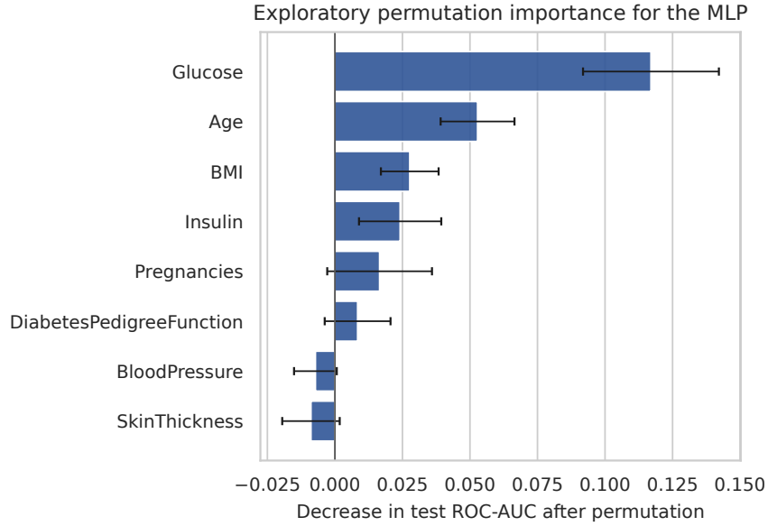
Fig. 7 Exploratory MLP permutation importance based on 30 shuffles per feature. Error bars show one standard deviation across shuffles. Negative values can occur from sampling variation.
