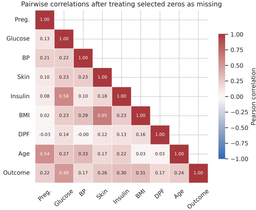
Fig. 3 Lower-triangle Pearson correlation matrix. Selected zeros in the five measurement fields were treated as missing and omitted pairwise. The plot was generated from the local dataset.
