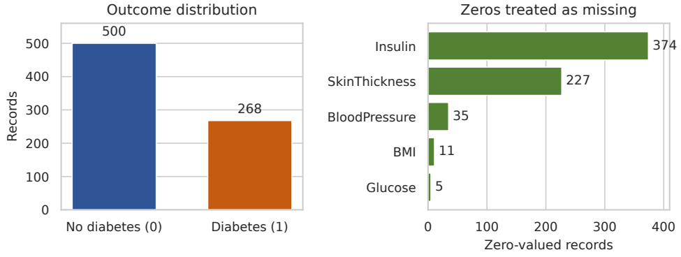
Fig. 2 Dataset audit: outcome counts and zeros treated as missing. Both panels were generated from the local CSV file.
