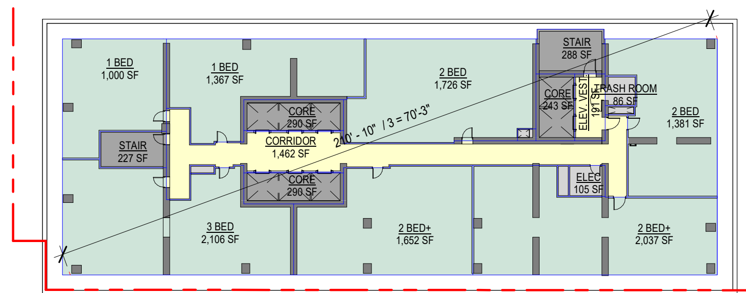
S - LEVELS 37 - 42 | BRANDED RESI SMALL 7 / A.005 | 1" = 30'-0"
