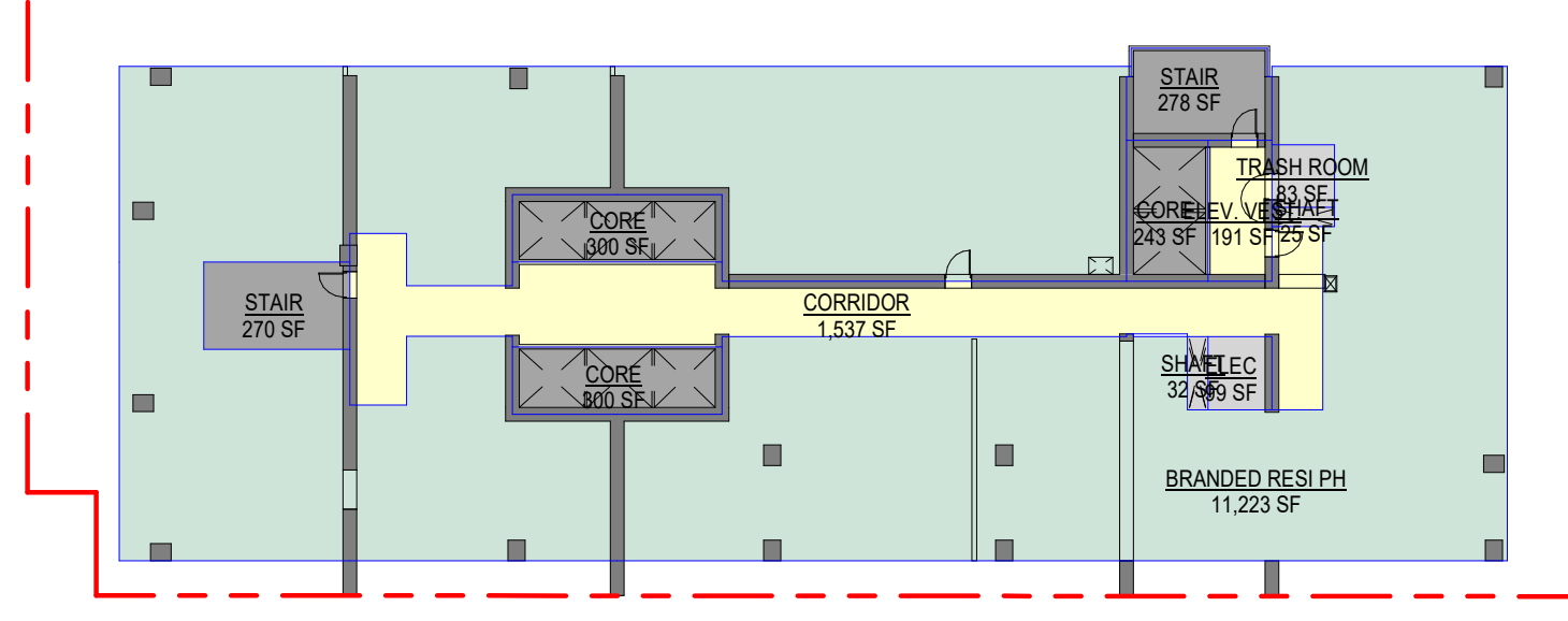
S - LEVEL 50 - BRANDED RESI PH 10 / A.005 | 1" = 30'-0"
