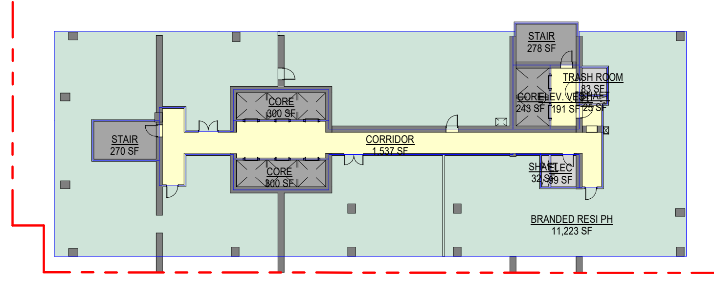
S - LEVEL 51 - BRANDED RESI PH 11 / A.005 | 1" = 30'-0"
