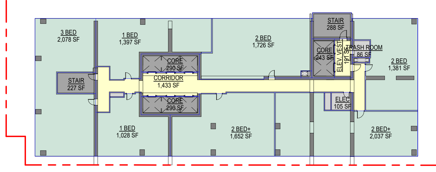
S - LEVELS 18 - 34 | BRANDED RESI SMALL 4 / A.005 | 1" = 30'-0"
