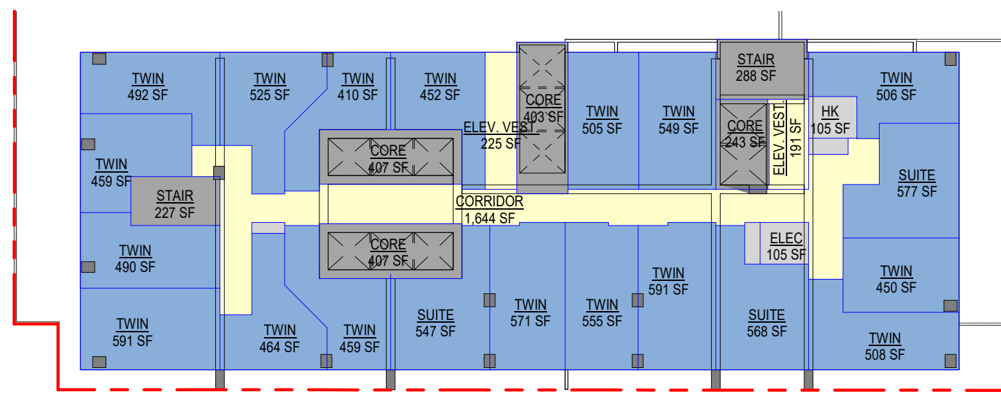
S - LEVELS 11 - 14 | HOTEL TYPE 1 1 / A.005 | 1" = 30'-0"
