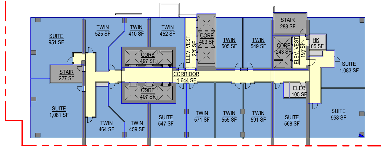
S - LEVELS 15 - 17 | HOTEL TYPE 2 2 / A.005 | 1" = 30'-0"
