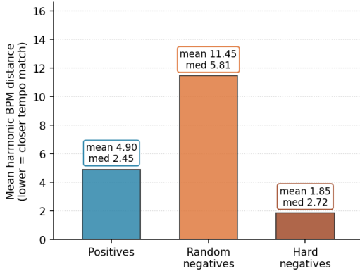
Figure 2: Mean harmonic BPM distance for positive pairs (real DJ transitions) and for negatives under each sampling regime. Random negatives sit at 11.45 BPM, well above the 4.90 BPM mean of positives, so harmonic BPM is a strong discriminator. Hard negatives, constrained within \pm 5 BPM of a positive anchor, drop to 1.85 BPM, tighter in tempo than the positives themselves. The cue therefore disappears under hard sampling, forcing the model to rely on non-tempo features.
