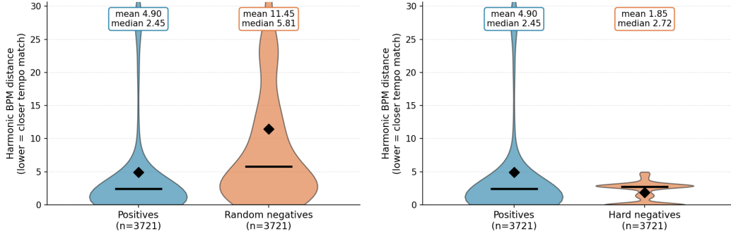
(a) Random negative sampling. Positive pairs have a mean harmonic distance of 4.90 BPM (median 2.45) compared to 11.45 BPM (median 5.81) for random negatives, providing clear separation between the two classes. (b) Hard negative sampling. The relationship inverts: hard negatives have a mean harmonic distance of 1.85 BPM (median 2.72), smaller than the 4.90 BPM mean of positive pairs. Because hard negatives are constrained within \pm 5 BPM of a positive anchor, they end up closer in tempo than the positive pairs themselves.
