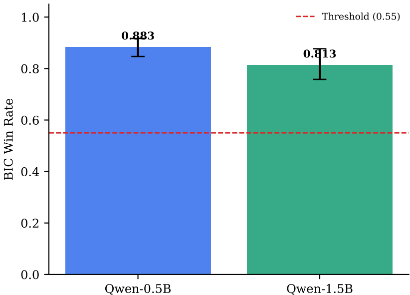
Staircase BIC Win Rate (100 problems, S=8, 95% CI)
