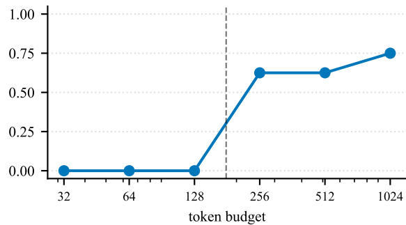
problem 52, \tau\text{-idx}=0 low- R^2 (noisy), R^2 = 0.50
