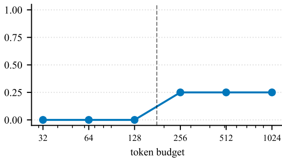
problem 25, \tau\text{-idx}=0 low- R^2 (noisy), R^2 = 0.45
