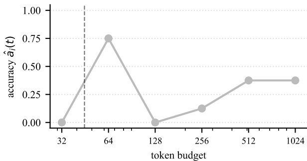
problem 98, \tau\text{-idx}=0 low- R^2 (noisy), R^2 = 0.21
