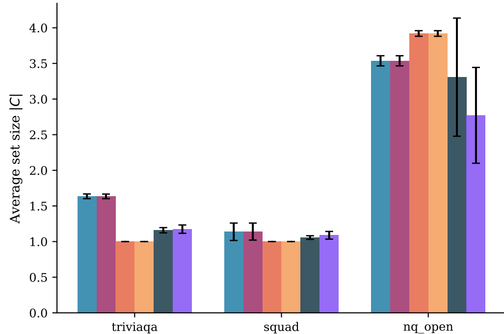
Prediction set efficiency
