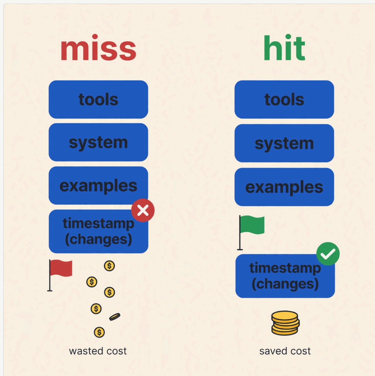
Figure 8. The breakpoint placement trap: a breakpoint after per-request content never hits; placed at the end of the static prefix, every request hits. Generated diagram.
