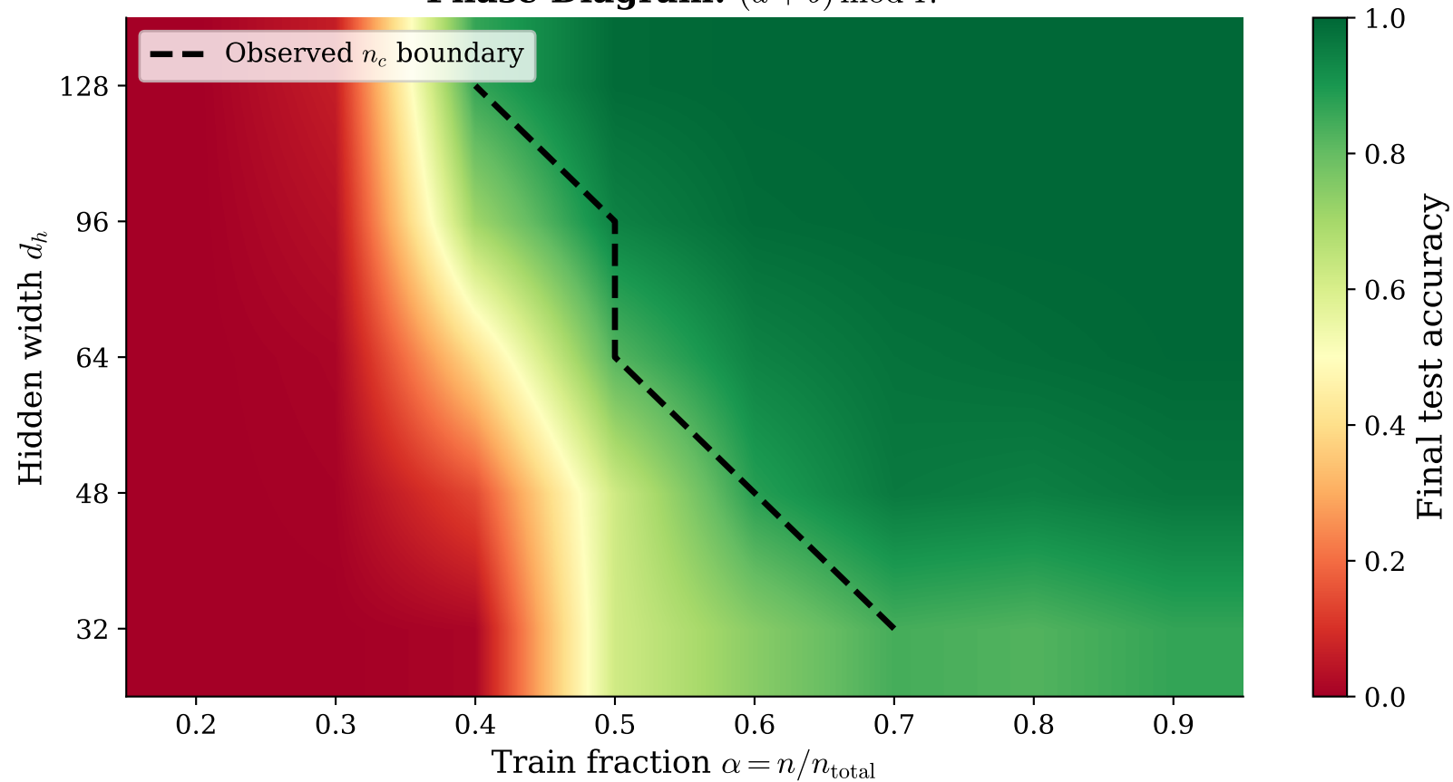
Phase Diagram: (a + b) \bmod 47
