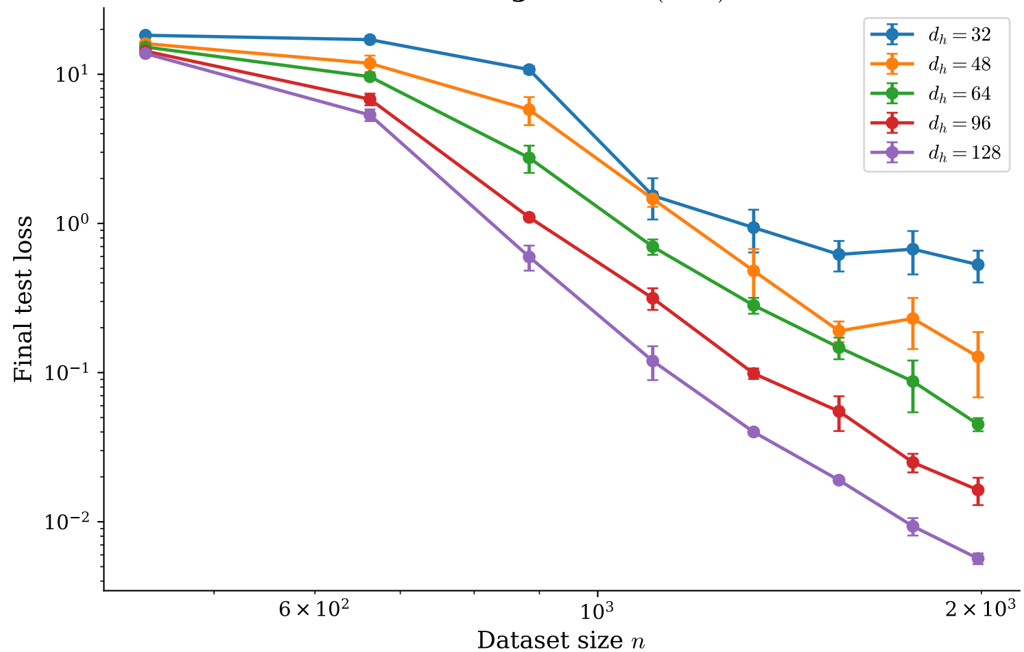
Neural Scaling Curves: (a + b) \bmod 47
