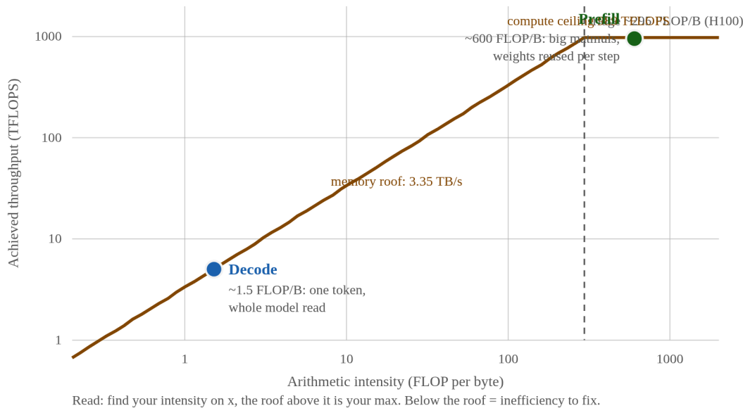
Figure 15.1. The roofline, drawn. Find your kernel's arithmetic intensity on the x-axis; the roof above it is the maximum throughput you can ever reach. Below the roof is inefficiency to fix. Decode sits far left ( \sim 1.5 FLOP/byte: one token, the whole model read, so it is bandwidth-bound); prefill sits far right ( \sim 600 FLOP/byte: big matmuls reuse weights, so it is compute-bound). The chart shows the bf16 roofline (ridge near 295 FLOP/byte); the fp8 dense ridge this pack quotes sits at 591.
