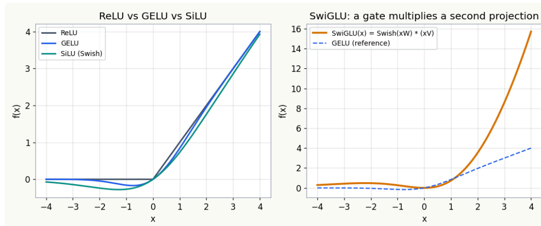
Figure 3.2. Activations compared. Left: ReLU, GELU, and SiLU (Swish) all bend near zero, but the smooth ones keep a small gradient for negative inputs. Right: SwiGLU is not one curve but a gate. It multiplies \text{Swish}(xW) by a second projection xV . The network learns which features pass.
