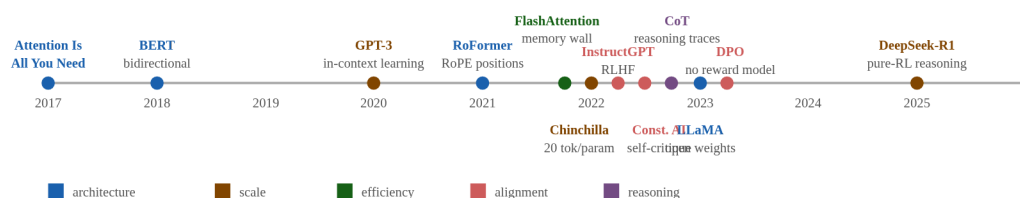
Figure 12.1. The spine in time. The 2022 cluster is the field's busiest year: FlashAttention (efficiency), Chinchilla (scale laws), InstructGPT and Constitutional AI (alignment), and chain-of-thought (reasoning) all landed at once. Mixture of Experts (2017/2024) runs underneath as the capacity thread.
