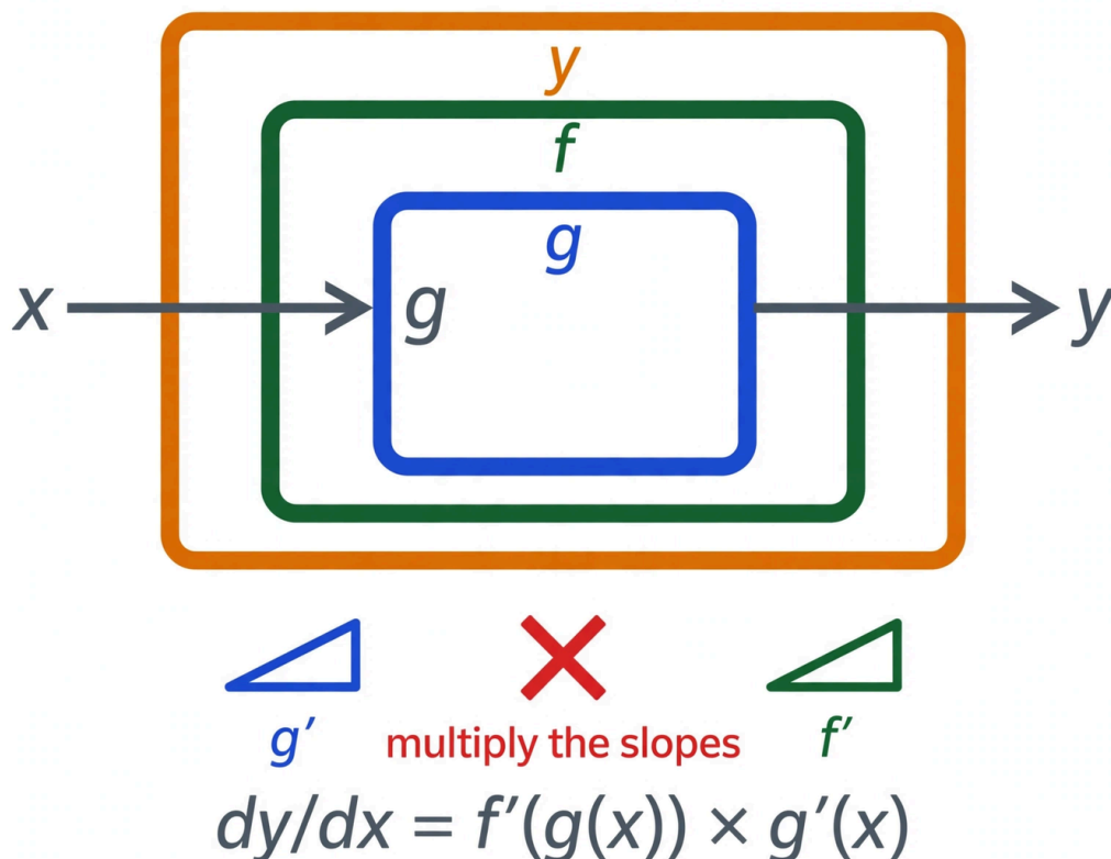
Figure 3.1. Backprop uses the chain rule. For nested functions y = f(g(x)) , the slope dy/dx is the product of the local slopes f'(g(x)) and g'(x) . Backprop applies this idea through every layer in reverse. Each weight learns its share of the error by multiplying the slopes along its path.
