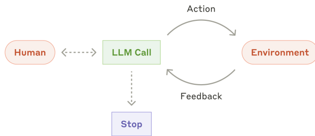
Figure 9.1. The agent loop. The LLM acts on the environment (tool calls), reads the feedback the environment returns, and repeats until it decides to stop. The human stays in the loop as an optional check, not as the engine.
