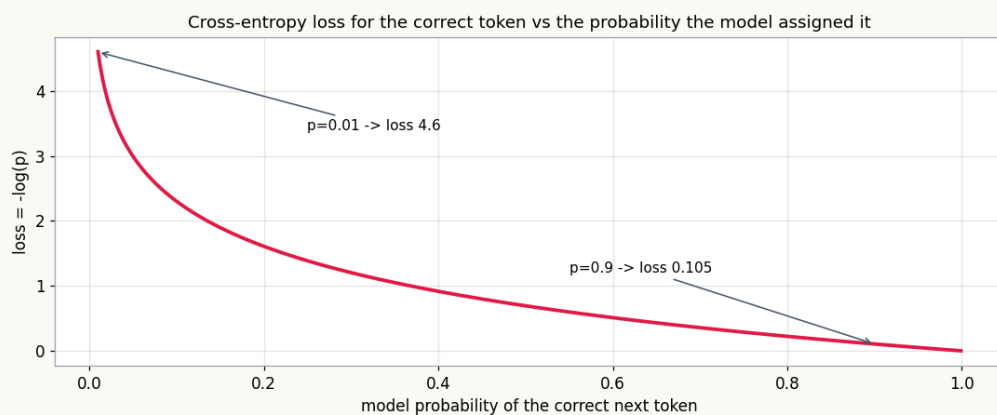
Figure 5.3. Cross-entropy for the correct token vs the probability the model assigned it: p = 0.01 costs 4.6 nats, p = 0.9 costs 0.105. A run's loss curve is this function averaged over tokens, which is why uniform over 32k starts at \ln(32000) = 10.37 .
