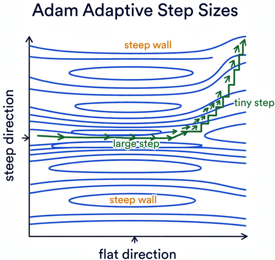
Figure 3.3. Adam adapts the step per parameter. Tiny steps for steep slopes. Large steps for flat slopes. Each parameter gets its own scale from its gradient history. In AdamW, weight decay is separate from the adaptive step.
