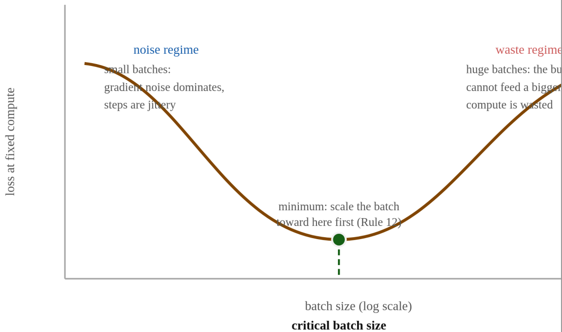
Figure 1.3. The U-curve behind Rules 10 and 12. At fixed compute, small batches drown in gradient noise (left wall). Large batches waste compute on a model size the budget cannot feed (right wall). The minimum is the critical batch size. Scale the batch toward it before touching the learning rate.
