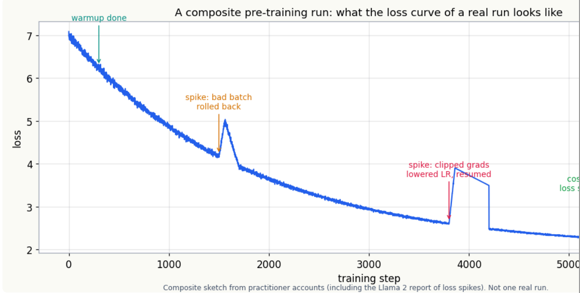
Figure 4.1. A composite pre-training run: what a real loss curve looks like. Warmup, a bad-batch spike (roll back), a clipped-gradients spike (lower the LR), then the cosine tail continues to fall. A healthy run is noisy but keeps descending.
