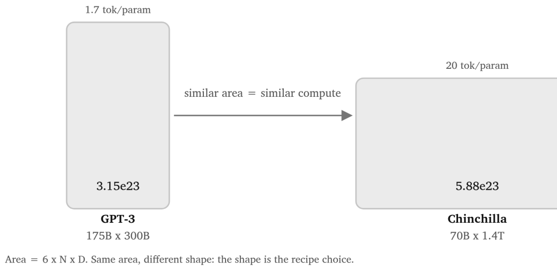
Figure 2.5. 6ND is an area. GPT-3 is tall and thin: 175B params times 300B tokens. Chinchilla is short and wide: 70B params times 1.4T tokens. Both areas land near 3 to 6e23 FLOPs. The shape is the recipe choice.
