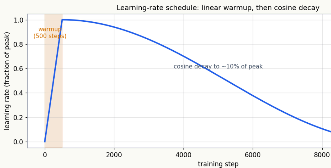
Figure 2.1. The standard LR schedule. Linear warmup first, then cosine decay to about 10 percent of peak. Warmup protects the early, unstable steps. The long decay is where most of the loss drop happens.
