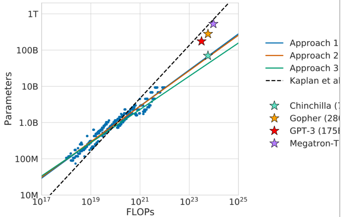
Figure 1.2. The Chinchilla tradeoff as parameters vs FLOPs. Three fitted approaches against the Kaplan et al. (2020) dashed line. Chinchilla (70B params, 1.4T tokens) sits on the efficient frontier. Gopher (280B) and GPT-3 (175B) sit off it. Rule 2 in one picture.
