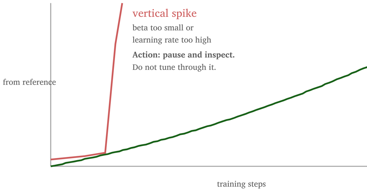
Figure A.7. KL from the reference over training steps. A steady climb with rising gold scores is healthy optimization. A vertical spike means the leash failed: beta is too small or the learning rate is too high. Pause and inspect. Do not tune through a spike.
