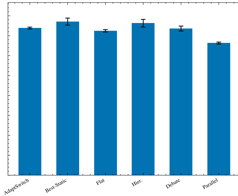
Planning Tasks
