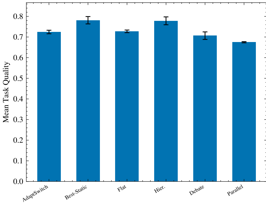
Coding Tasks
