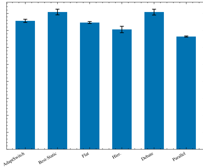
Reasoning Tasks
