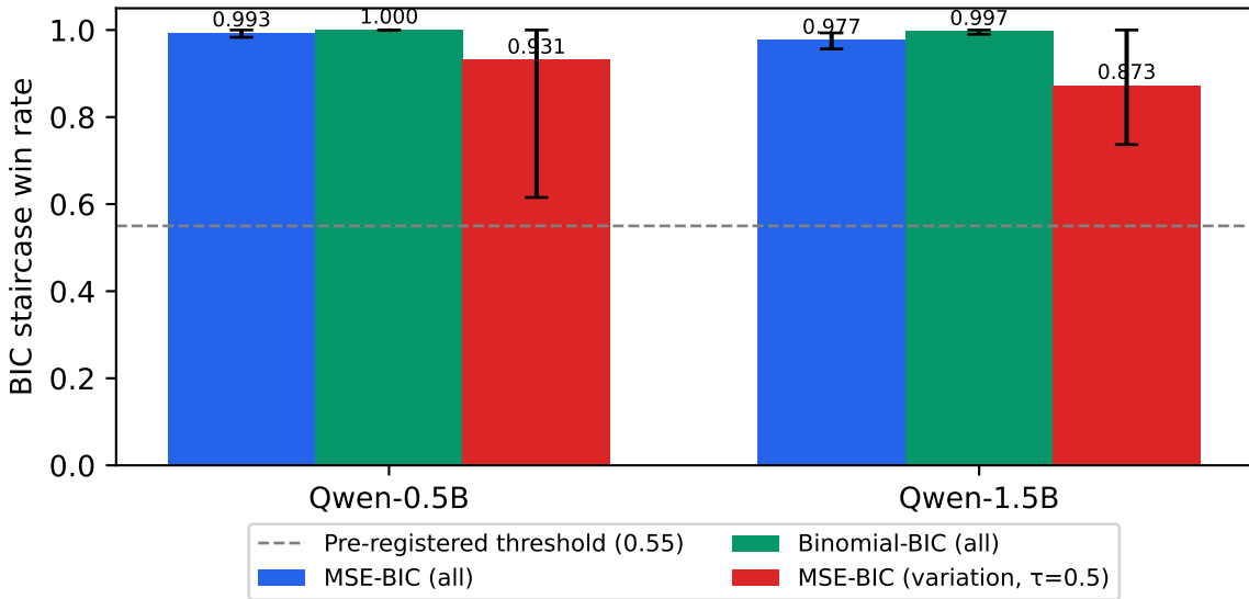
Per-problem staircase wins on real GSM8K
