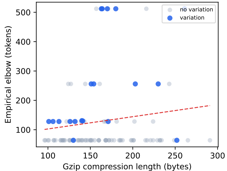
Gzip vs elbow (Qwen-1.5B, \tau=0.5 ) \rho=0.143 , 95% CI [-0.015, 0.321], p=0.16
