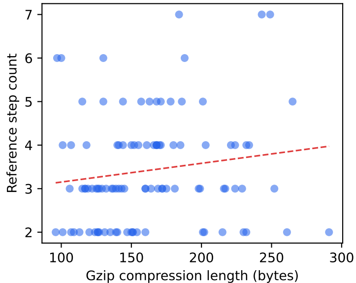
Gzip vs step count (n=100) \rho=0.147 , 95% CI [-0.088, 0.383], p=0.14
