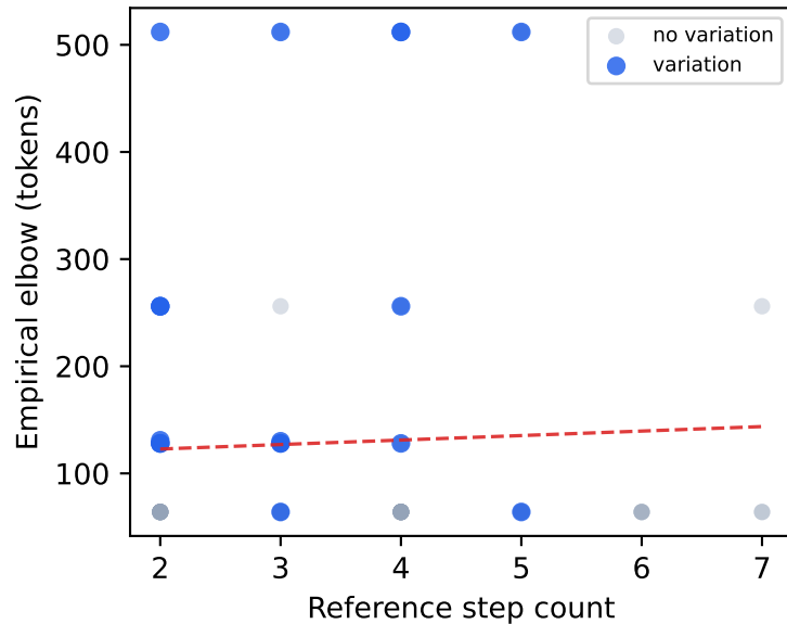
Step count vs elbow (Qwen-1.5B, \tau=0.5 ) \rho=0.042 , 95% CI [-0.161, 0.234], p=0.68
