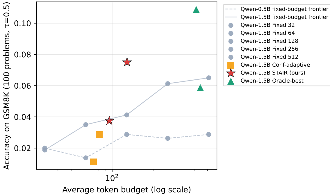
Real-data Pareto: accuracy vs. average token cost
