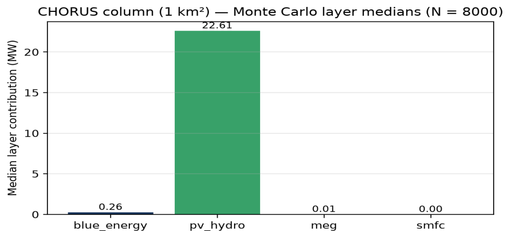
Figure 6. Median layer contributions.
