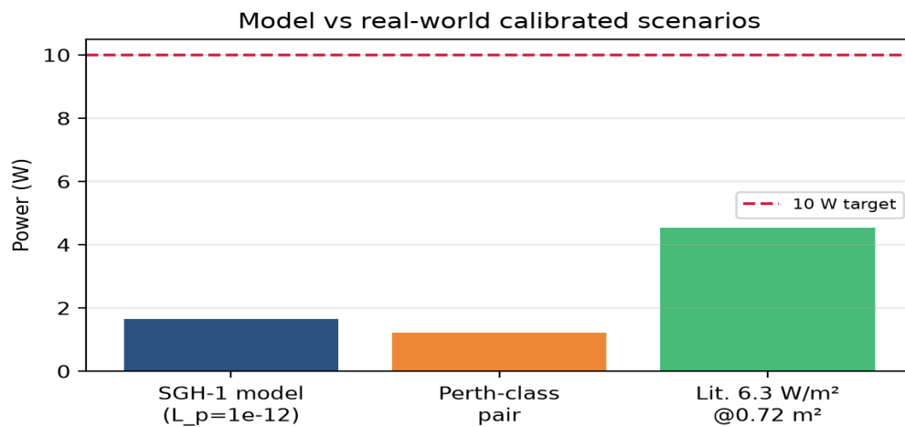
Figure 2. SGH-1 model power vs Perth-class pair vs literature 6.3 W/m 2 reference.
