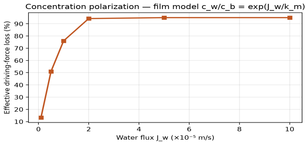
Figure 7. Driving-force loss versus water flux.
