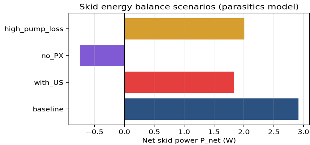
Figure 10. Net power scenarios with pump and PX model.
