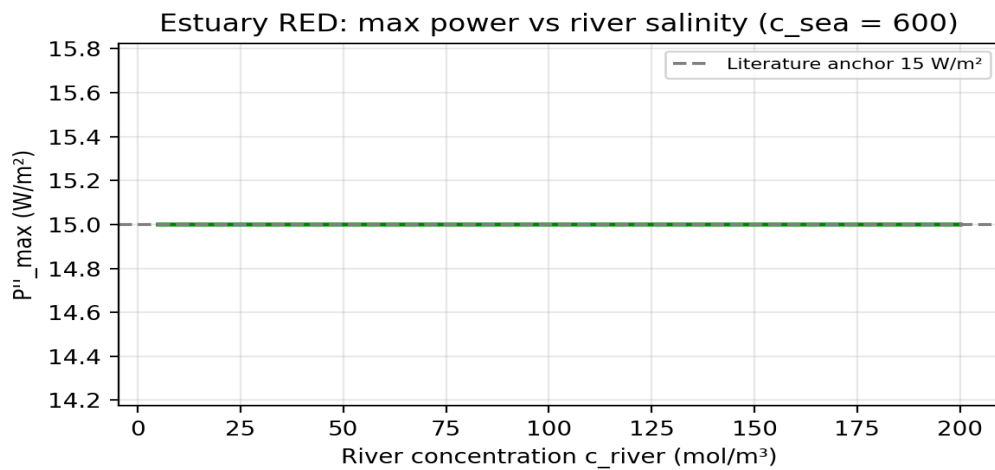
Figure 8. Estuary RED P''_{\text{max}} versus c_{\text{river}} .
