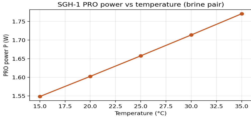
Figure 9. PRO power versus temperature.
