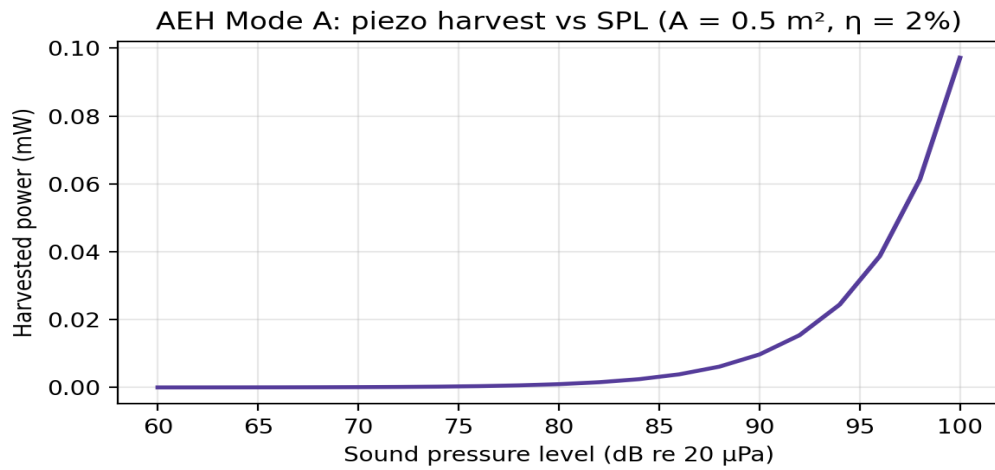
Figure 7. Mode A harvest versus SPL.
