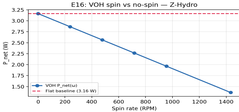
Figure 16. Z-Hydro: P_{net} versus spin rate with flat baseline.
