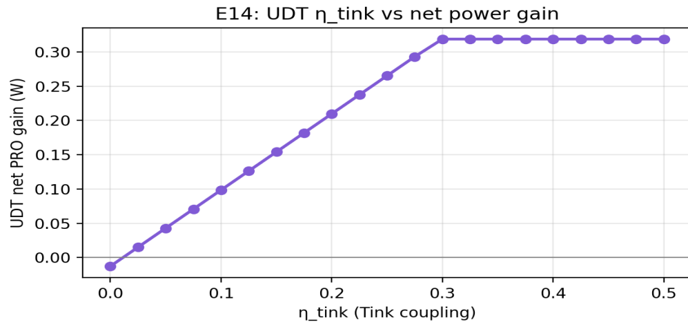
Figure 14. UDT coupling efficiency vs net PRO gain.
