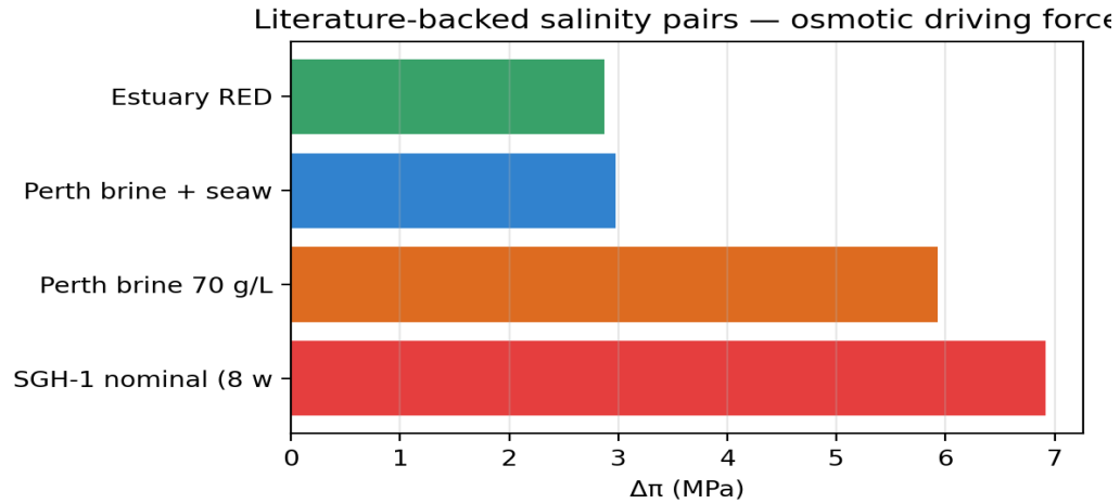
Figure 1. Osmotic pressure difference for literature-backed feed/draw pairs.
