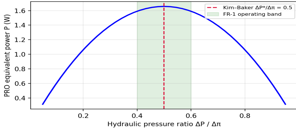
Figure 3. PRO power versus \Delta P / \Delta \pi with FR-1 band and Kim-Baker optimum.
