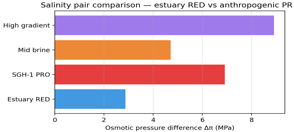
Figure 5. \Delta\pi across estuary RED and anthropogenic PRO pairs.
