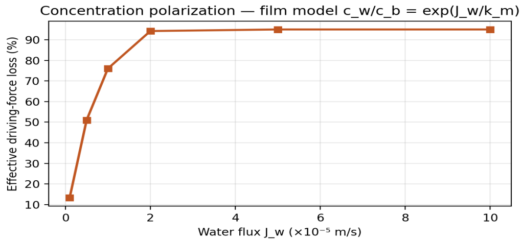
Figure 7. Driving-force loss versus water flux.
