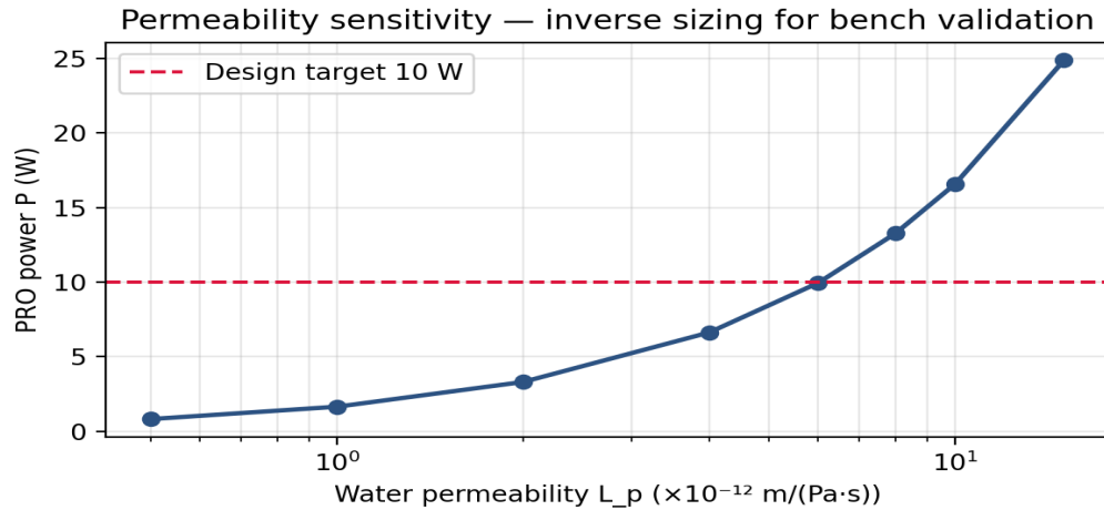
Figure 4. Power versus water permeability L_p .
