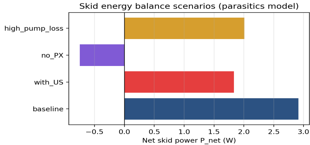
Figure 12. Net power scenarios with pump and PX model.
