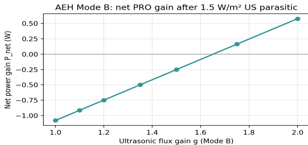
Figure 8. Net power versus flux gain g .
