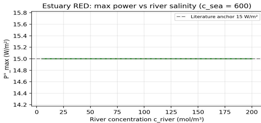
Figure 10. Estuary RED P''_{\text{max}} versus c_{\text{river}} .
